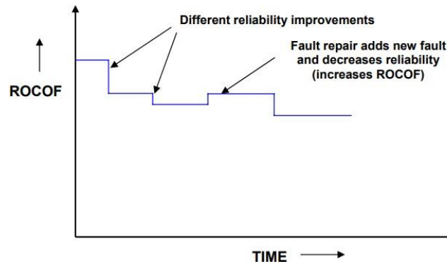
Figure 11.2: Random Step Function Model of Reliability Growth.
