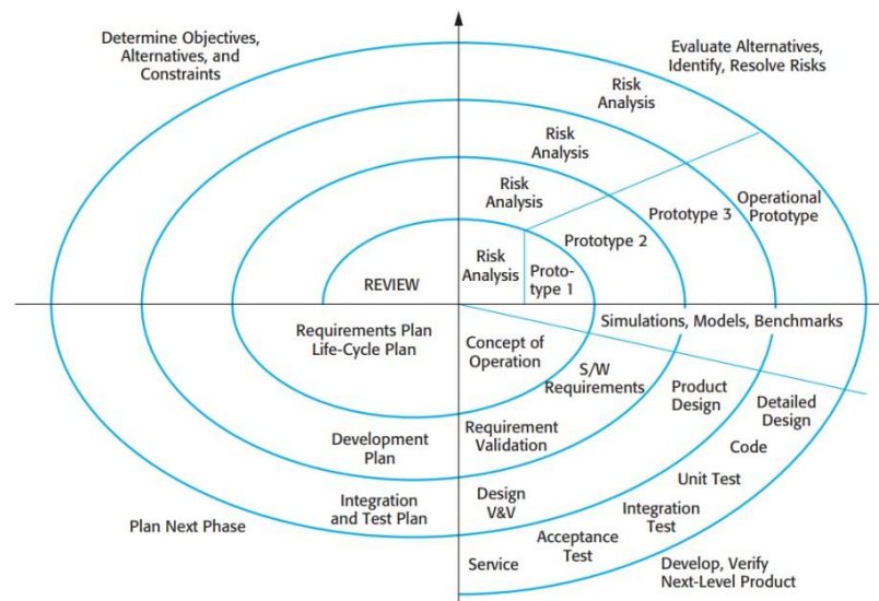
Figure 6: Spiral lifecycle Model
